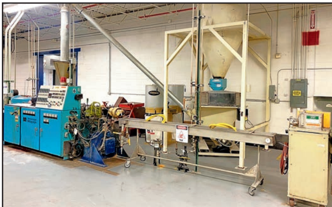
REGRIND/PELLETIZER SYSTEM
