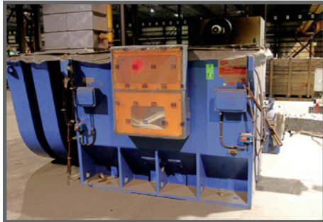
5000 HP WEG MGF 12807 3-PHASE INDUCTION MOTOR
