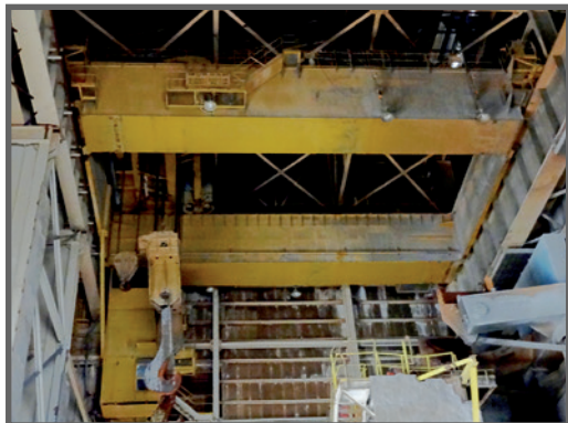
265 TON MORGAN 265/50 AUXILIARY 67' SPAN BRIDGE CRANE
