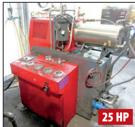
PREMIER MILL HM-15VSD 25 HP MEDIA MILL
