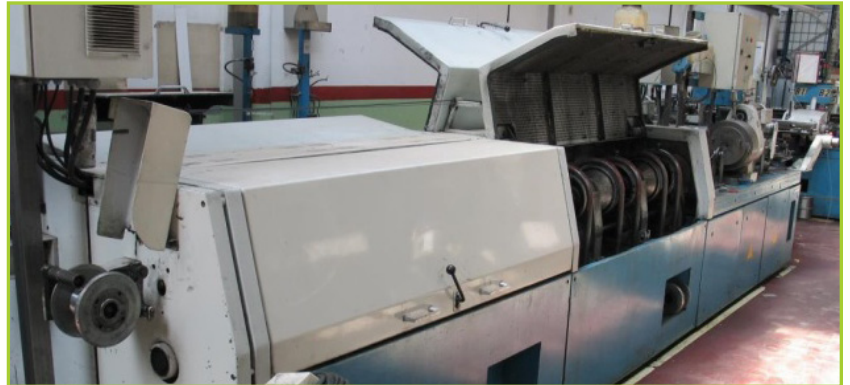
BARMAG DV2 SECTION 1: 6+1 WIRES (CURRENTLY AT 1X0,591 + 6X0,541 FOR GALVANISED), 26,854 TOTAL RECORDED HOURS, WITH FELSS HE18-D HAMMERING ATTACHMENT (S/N 2813. YEAR 2000), VARIABLE SPEED DRIVE. SECTION 2: 6+1 WIRES (CURRENTLY AT 1X0,6 + 6X0,54 FOR SS), 65,265 TOTAL RECORDED HOURS, WITH FELSS HE16-D HAMMERING ATTACHMENT (S/N 2931. YEAR 2001). VARIABLE SPEED DRIVE. WIRE DIA RANGE (FOR STEEL OR STRAND STEEL WIRE): 0,1-0,38 MM. SPEED: 8000 RPM
