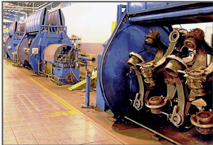
KRUPP 54-WIRE STAR TYPE RIGID STRANDER
