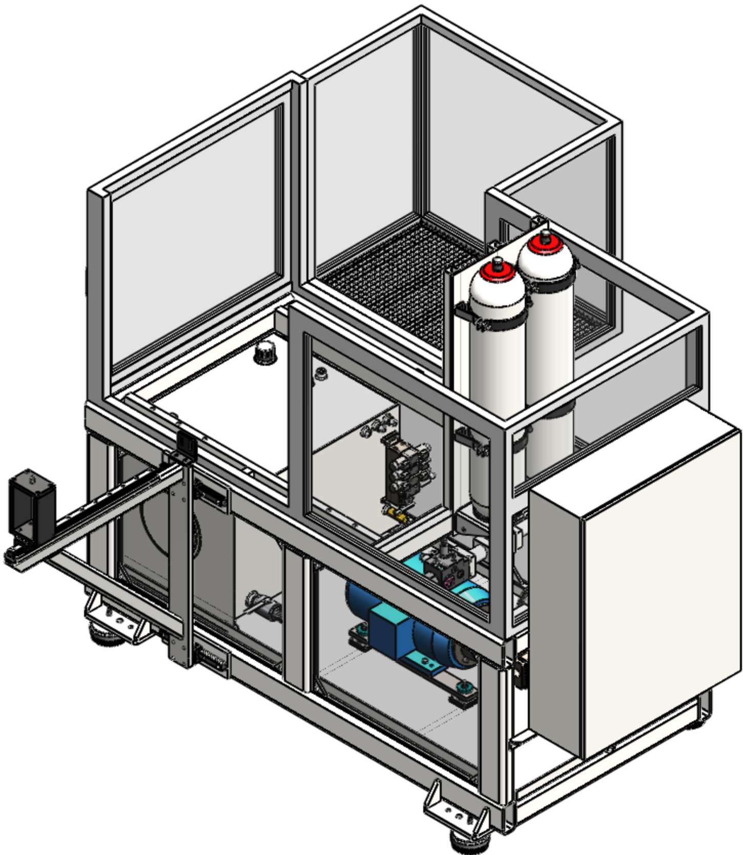
Frame, HPU, and Guard Assembly See Sheet 2
