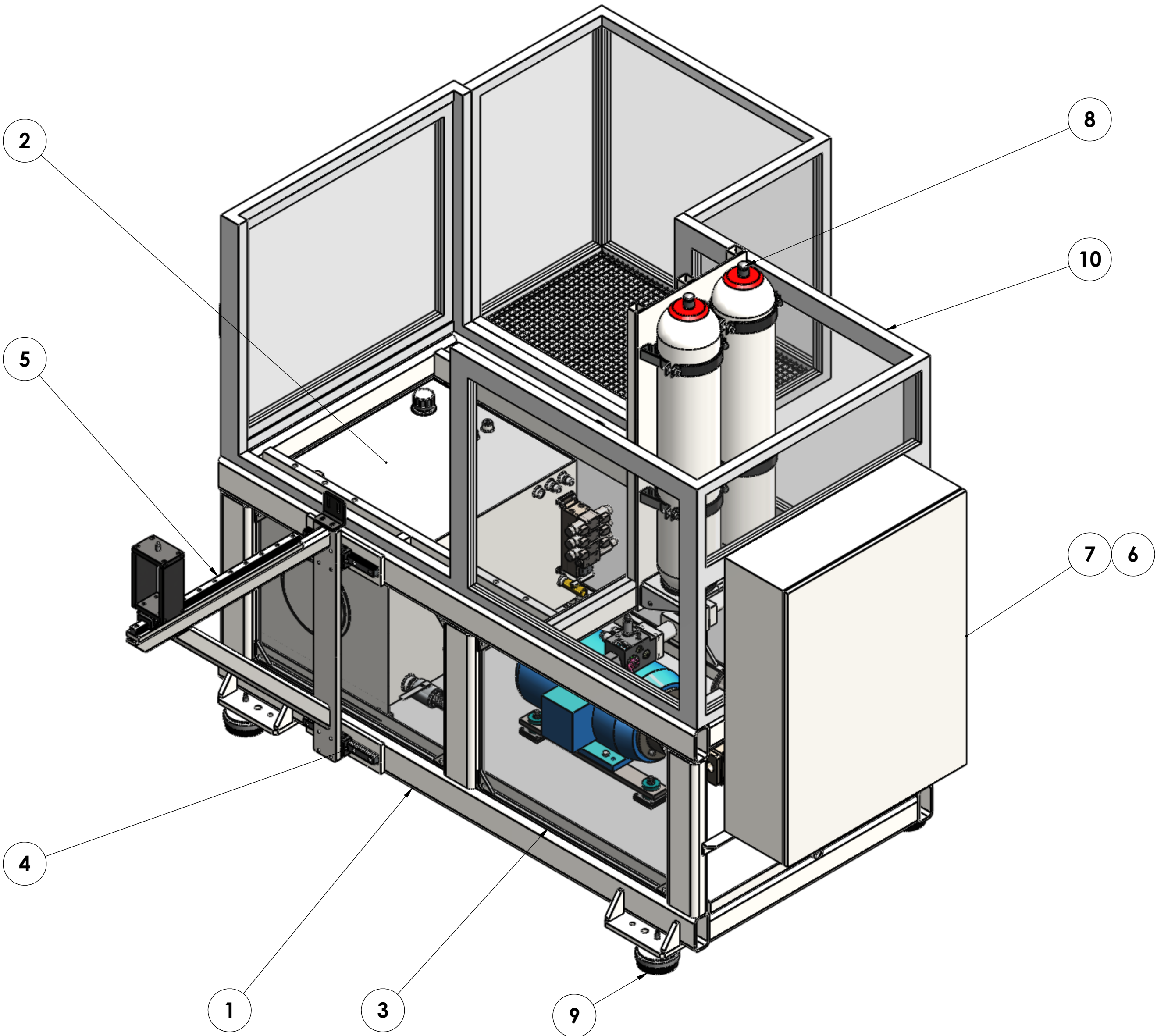
Frame, HPU, and Guard Assembly
