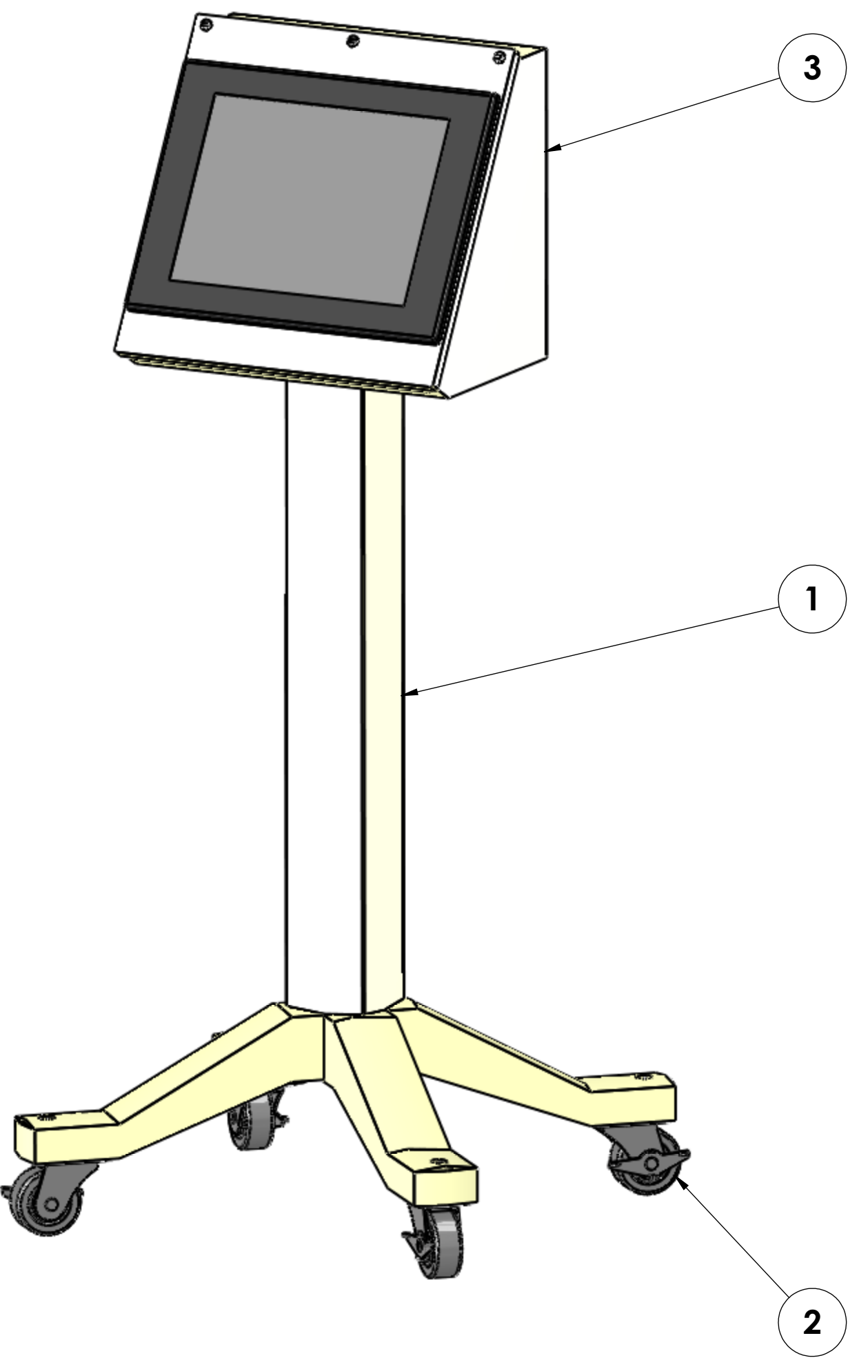
HMI Pedestal Assembly
