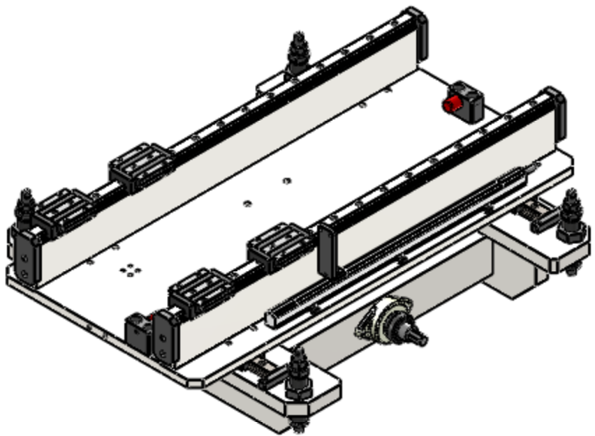
Carriage Subassembly See Sheet 3
