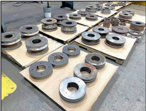
ROUND R6S ANGLE BENDING ROLL
