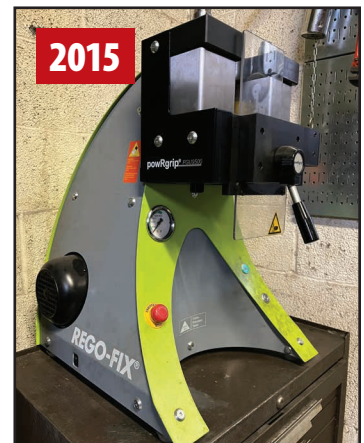
REGO-FIX POWRGRIP PGU9500 AUTOMATIC TOOL CLAMPING SYSTEM
