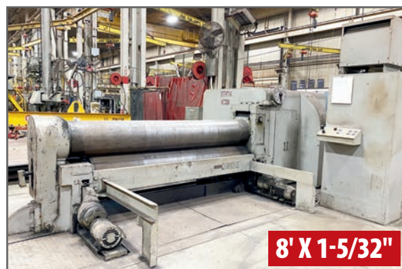
BERTSCH 14-E INITIAL PINCH PLATE ROLL
