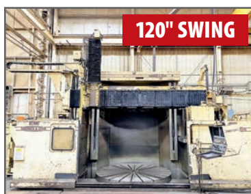
G & L 108-VTC CNC VERTICAL BORING MILL
