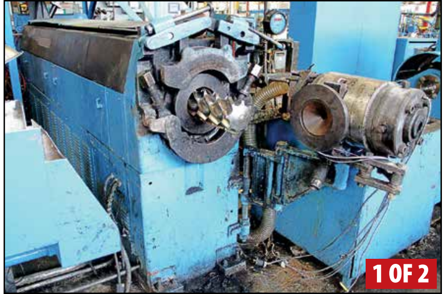
DAVIS STANDARD 600S 6" 24:1 L/D EXTRUDER
