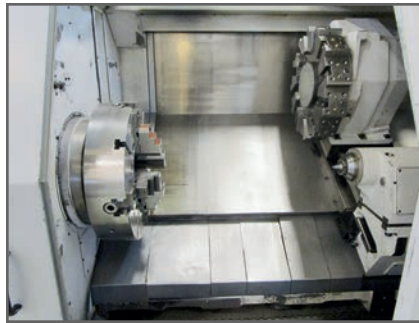
OKUMA LB35-II WORK ENVELOPE
