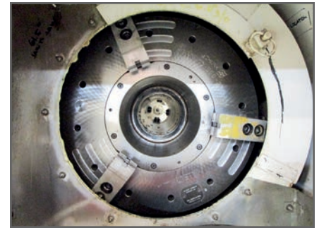
OKUMA LB35-II "SCHUNK" REAR CHUCK
