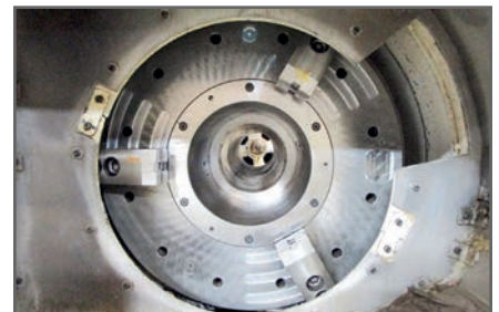
OKUMA LB35-II "SCHUNK" REAR CHUCK
