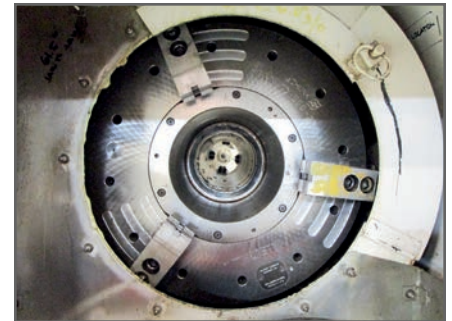
OKUMA LB35-II "SCHUNK" REAR CHUCK
