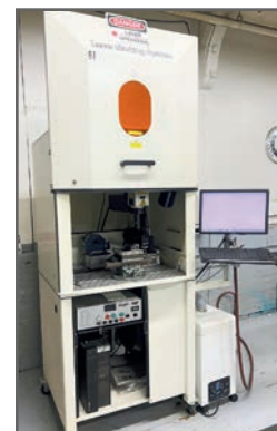
TELESIS 16" X 16" LASER MARKING SYSTEM
