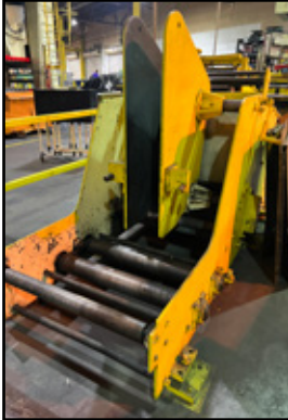
ROWE 8,000 LB X 15" FEED LINE
