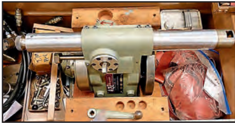
CLIMAX JS JOURNAL SQUIRREL PORTABLE LATHE
