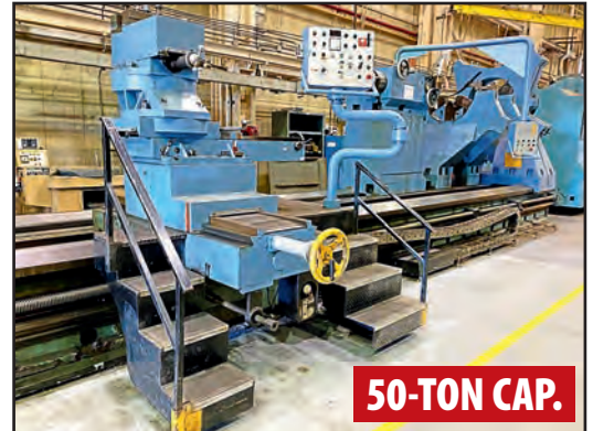
GIANA GFP-24 129" X 421" CARRIAGE, STEADY RESTS AND TAILSTOCK
