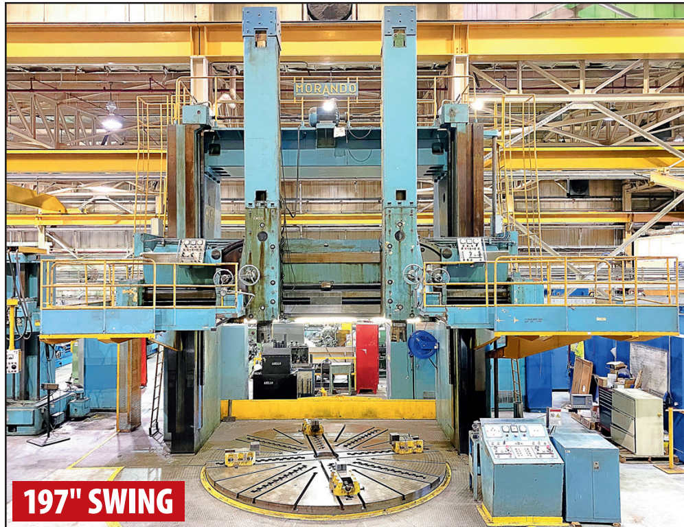
MORANDO KS 42/50 VERTICAL BORING MILL
