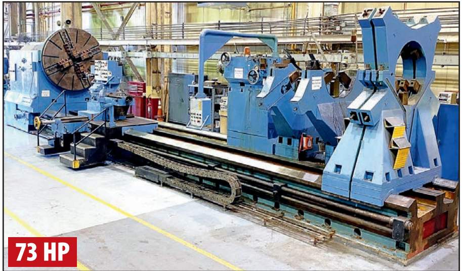
GIANA GFP-24 129" X 421" HD LATHE
