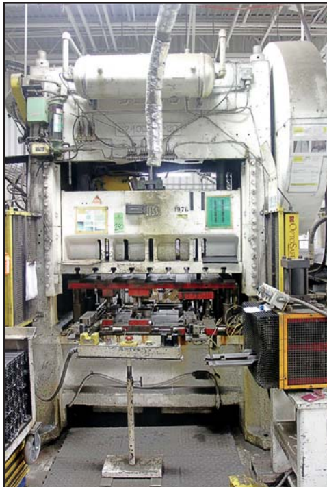
100-TON BLISS S2-100-60-30 STRAIGHT SIDE DOUBLE CRANK PRESS
