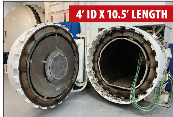
THERMAL EQUIPMENT CORP. AUTOCLAVE
