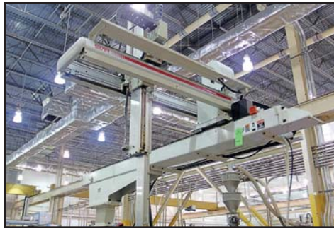
STAR AUTOMATION TW-1400FM-3 ROBOT
