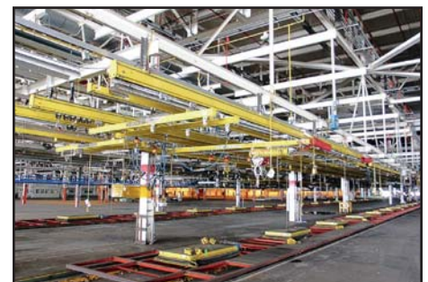
SKILLET LINE W/(40) LIFT TABLES
