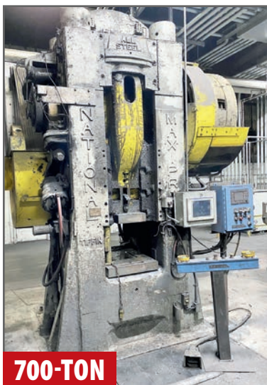
NATIONAL NO. 3 MAXI FORGING PRESS
