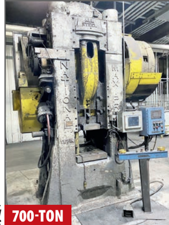
NATIONAL NO. 3 MAXI FORGING PRESS
