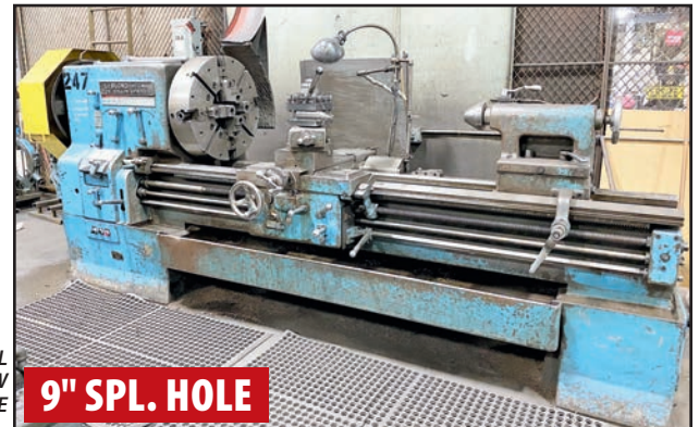
LEHMAN HYDRATROL 28" X 120" HOLLOW SPINDLE LATHE
