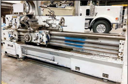
LODGE & SHIPLEY 2013/17 POWERTURN 26" X 120" ENGINE LATHE
