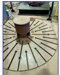
Clad Unit #4: A&N Plant Model RC4X3.75 Cladding Machine (S/N 2558), Arc Specialties Hot One Solid State Hotwire Power Supply (S/N 0999-96006), 100" dia. table, 122" boom vert. trvl, 69" hor. trvl, 218" overall ht., Esab 350 MPI MIG Welder, DC TIG Arc Starter, Best Welds Welding Torch Water Cooler
