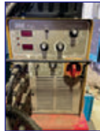
Clad Unit #1: A&N Plant Model RC40X3.75 Cladding Machine S/N 3160/3202), Arc Specialties Hot One Solid State Hotwire Power Supply (S/N 1018-20031), 100" dia. table, 118" mm boom vert. trvl, 69" boom hor. trvl, 213" overall ht., Thermal Arc DC TIG Arc Starter, Esab 350 MPI MIG Welder (S/N WE-J045029), Bernard 3500SS TIG/MIG Welding Torch Water Cooler
