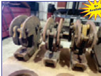
Heavy Duty Metal Plate Grips, assorted sizes, weight capacities
