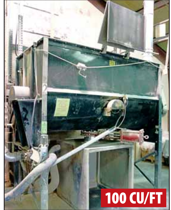
MUNSON RIBBON BLENDER
