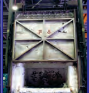
F3, 2200 Deg. F, 160" W x 118" H x 106" D, natural gas, 4 burners, fiber lined, Honeywell controls
