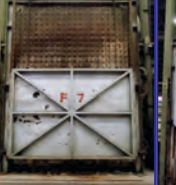
F7, 2200 Deg. F, 160" W x 118" H x 106" D, natural gas, 4 burners, fiber lined, Honeywell controls
