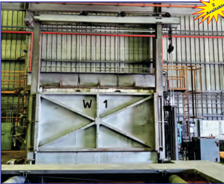
W1 / W2 , 1850 Deg. F, 166" W x 76" H x 94" D, natural gas, 4 burners, fiber lined, Honeywell controls
