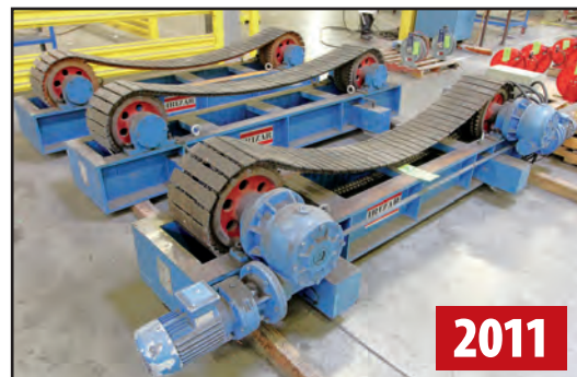
IRIZAR CWR-40 POWER CHAIN-TYPE TANK TURNING ROLLS
