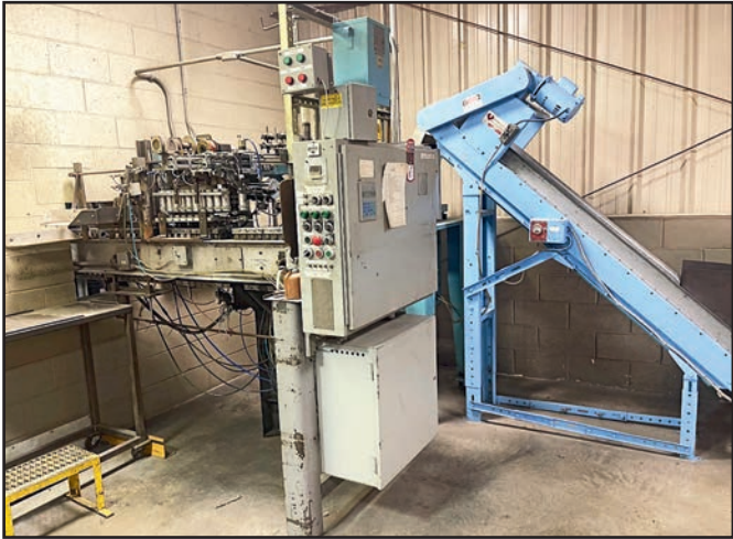
DUAL SIDE DRILL STATION W/VIBRO BLOCK 30L FEEDER
